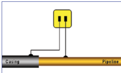
Type - CA - For checking the electrical isolation between pipeline and casing as well as pipe-to-soil potential measurements
