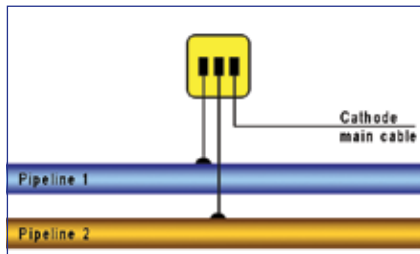
Type - CJB - For connection of pipelines or structures with different current requirements using diodes and variable resistors
