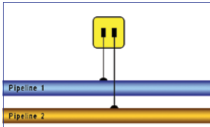
Type - PB - For electrical connection of isolated pipelines using a variable resistor as well as pipe-to-soil potential measurements
