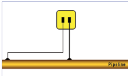
Type - C - For measurement of pipeline current as well as pipe-to-soil potential measurements
