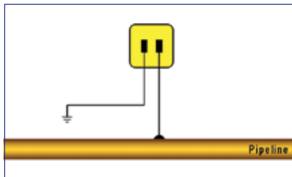
Type - E - For earthing the pipeline interfered by induced high voltage lines by means of lightning arresters as well as pipe-to-soil potential measurements
