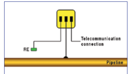
Type - RM - For remote monitoring of pipe-to-soil potential using transmitters
