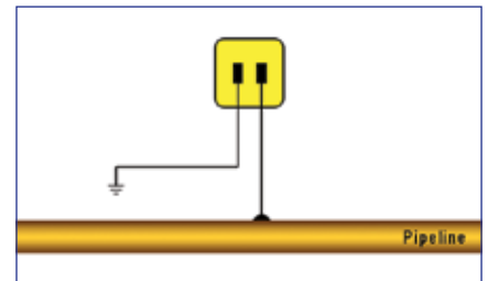
Type - L - For earthing the pipeline interfered by induced high voltage lines by means of diodes and condenser cascades as well as pipe-to-soil potential measurements
