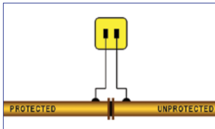
Type - I - For checking the efficiency of insulating flanges or joints as well as pipe-to-soil potential measurements
