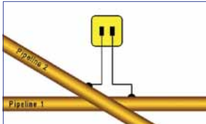
Type - CR - For checking interference between the protected pipeline and other pipelines or structures as well as pipe-to-soil potential measurements
