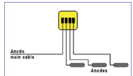
Type - AJB - For measuring and adjusting output current of individual string anodes using shunts and variable resistors
