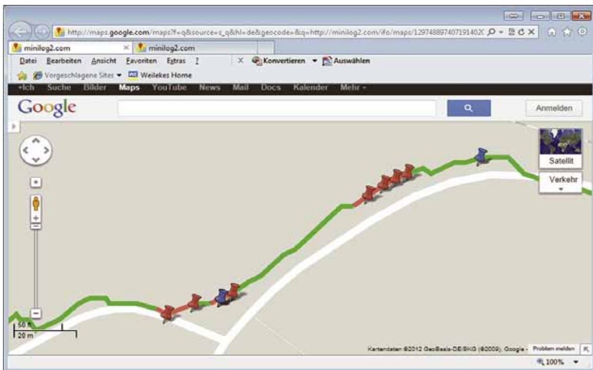
DCVG measurement export to Google® Maps for defect localization
